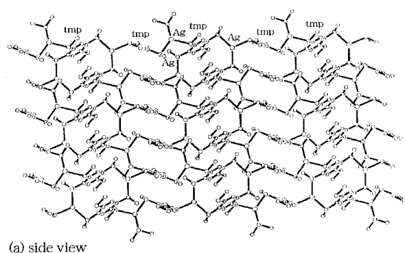
Fig. 2 Molecular structure of complex 1: (a) side view, (b) molecular packing.
